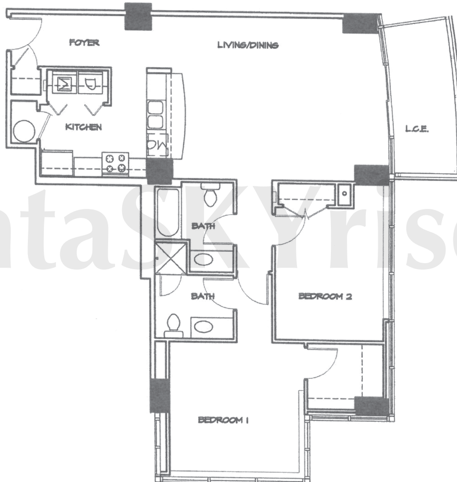
1 FLOOR PLAN - UNIT TYPE 'S' SCALE 1/8" = 1'-0" 2 BEDROOM, 2 BATH
